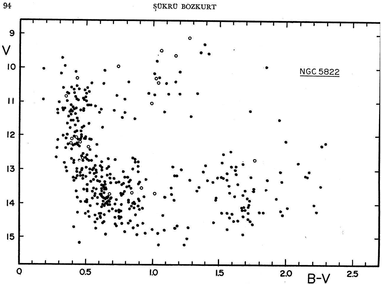
FIG. 4. Color-magnitude diagram for the region of NGC 5822. Stars with photoelectric magnitudes are shown by open circles, and those with photographic magnitudes filled circles.
