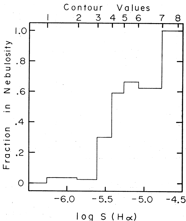
FIG. 1. Fraction of observed points by Reynolds et al. (1974) that are inside detectable nebulosity in the RPSS, for each of the nine contour intervals defined by them. The equivalent surface brightness corresponding to each contour value is also given.
