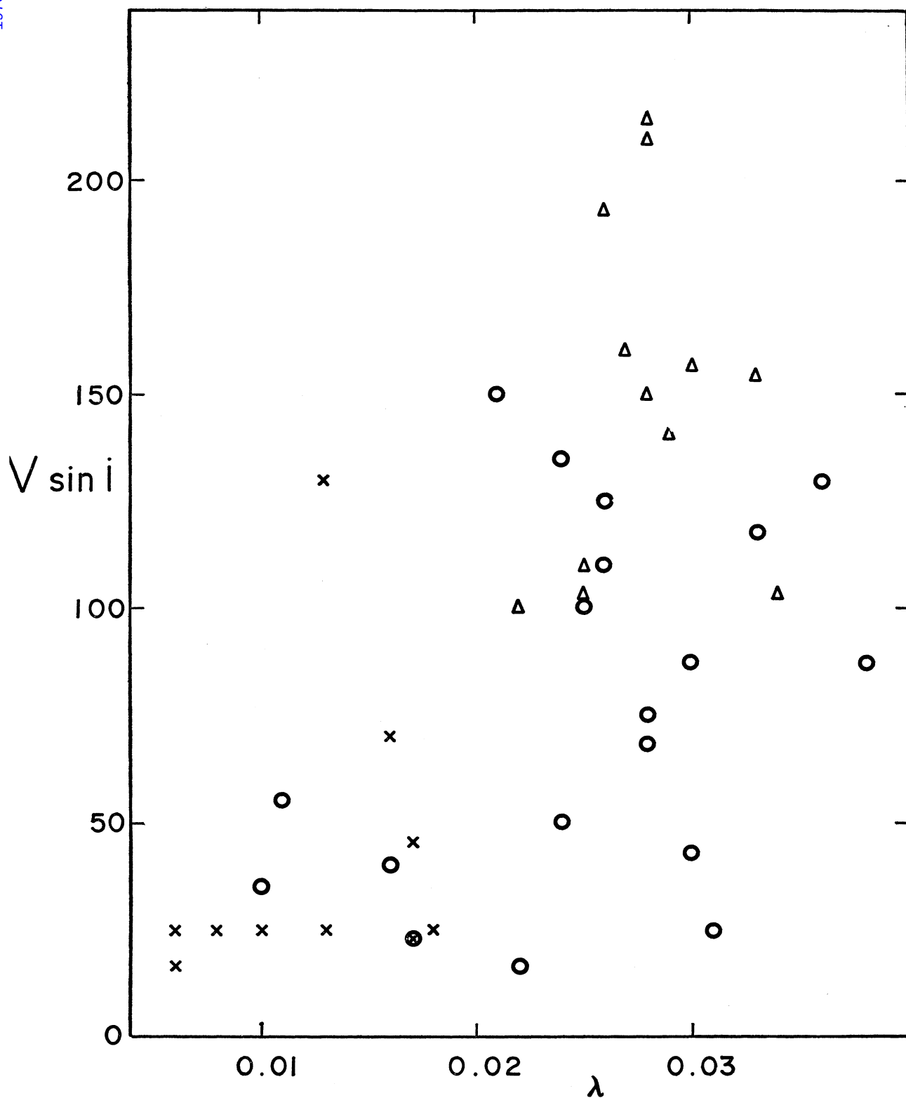
FIG. 7. The (\lambda, V \sin i) -array for the Hyades stars. The symbols have the same meaning as in Fig. 2.
