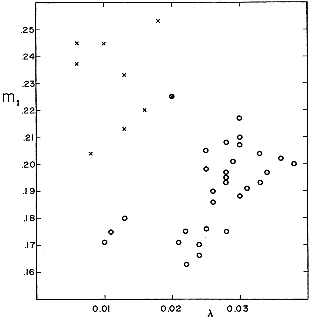
FIG. 5. The (\lambda, m_1) -array for the Hyades stars. The symbols have the same meaning as in Fig. 2.
