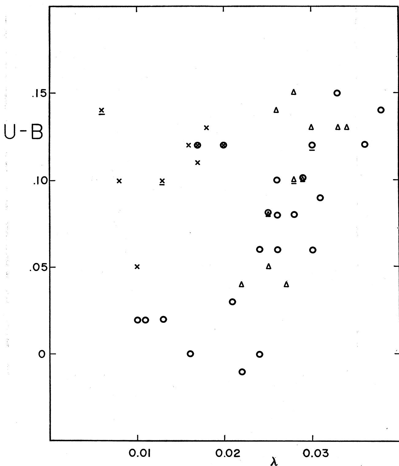
FIG. 6. The ( \lambda , U-B)-array for the Hyades stars. The symbols have the same maning as in Fig. 2.
