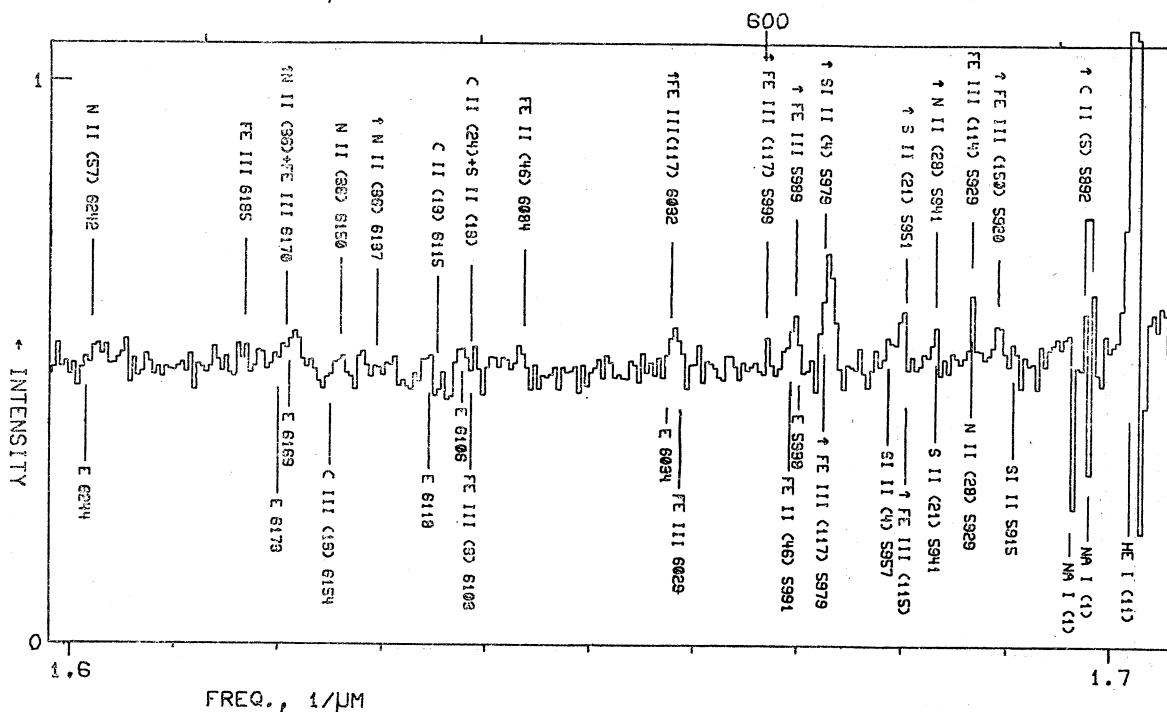
FIG. 5. The spectrum of P Cyg from 4800-10200 Å.
