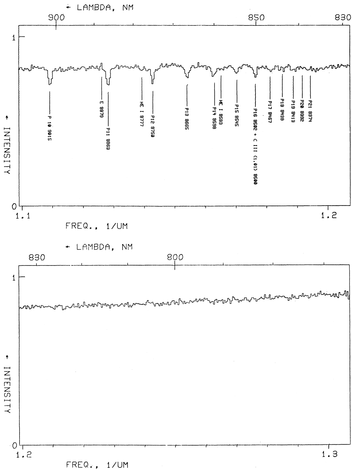
FIG. 4. The spectrum of \zeta Ori from 4800-10200 Å.
