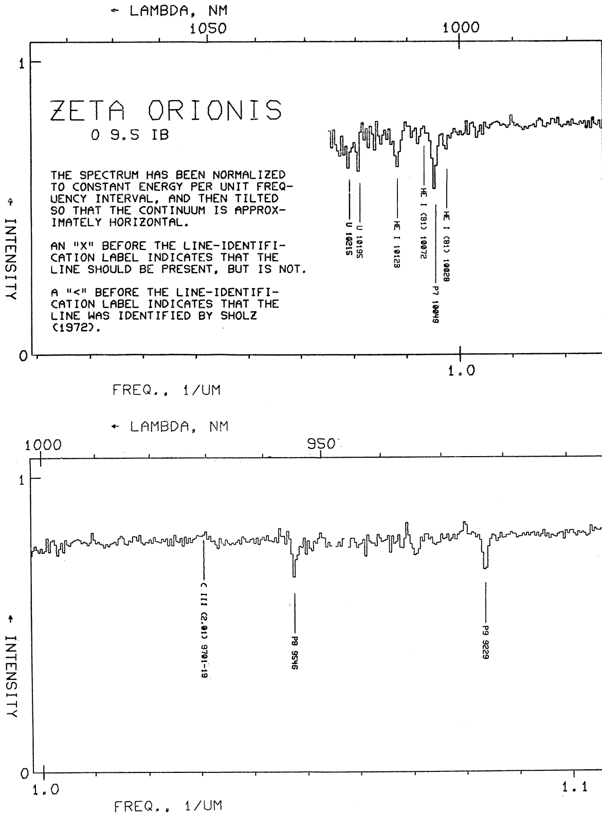
FIG. 4. The spectrum of \zeta Ori from 4800-10200 Å.
