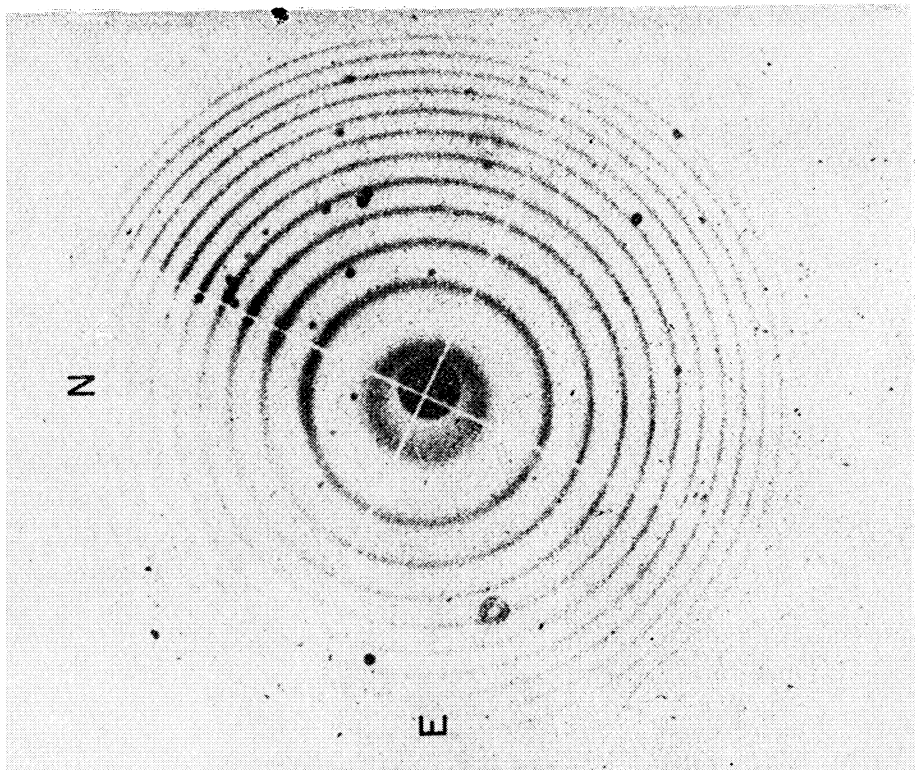
FIG. 2. An image tube H\alpha interferogram of S 140 using an étalon with an inter-order separation of 190 \text{ km s}^{-1} .
