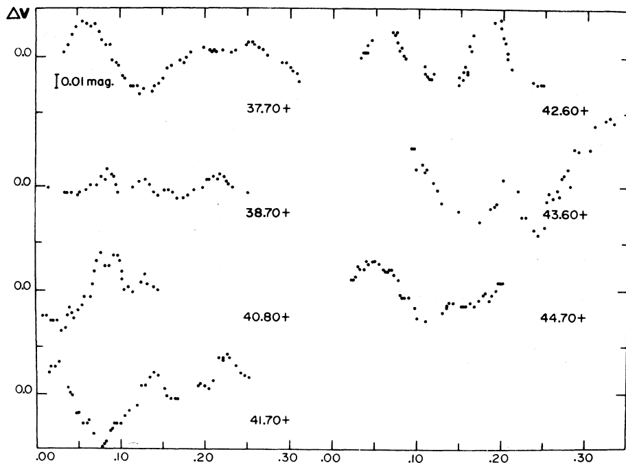
Fig. 2. Light curves of HR 4715.
