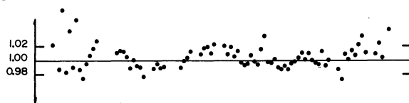
Fig. 1. The comparison of the absolute fluxes for Vega by Tüg, White and Lockwood, and those of this paper, F(\text{TWL})/F(\text{J}) . The wavelength is 9 000 Å at the left edge of the figure; 4 000 Å at the right edge.
