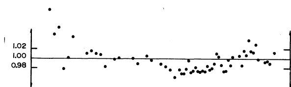
Fig. 2. The comparison of the absolute fluxes for 109 Vir by Tüg, White and Lockwood, and those of this paper, F(\text{TWL})/F(\text{J}) . The wavelength is 9 000 Å at the left edge of the figure; 4 000 Å at the right edge.
