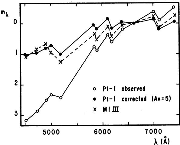
Fig. 3. Comparison of continuum fluxes of the symbiotic star Pt-1 to the M1 III unreddened star X Peg, normalized at \lambda 620 . Open circles correspond to the observed fluxes of Pt-1. Filled circles correspond to the best fit of the observations of the blue continuum of Pt-1 to X Peg assuming the normal reddening law; this fit yields A_V = 5 mag, or C(H\beta) = 2.36 .
