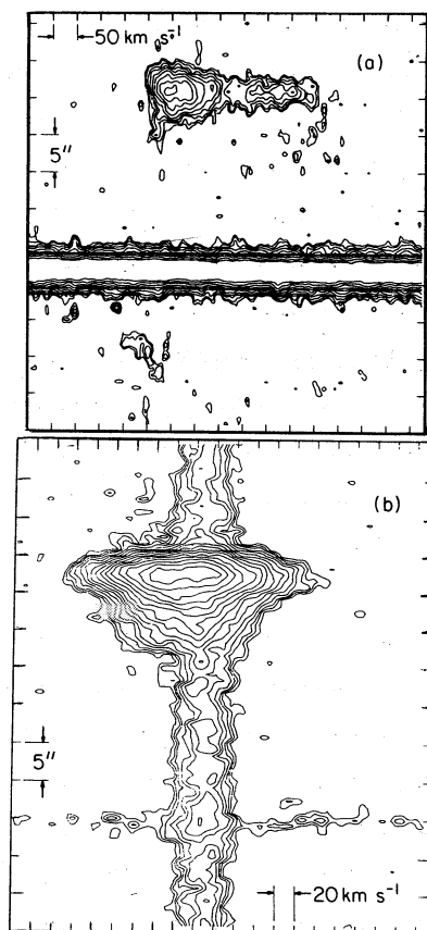
Figure 1. Contour lines showing line flux densities of the [N II] 6583 line in H-H 32(a) and the H\alpha line in H-H 1(b). The ordinate corresponds to the geometrical coordinate along the spectrograph slit, the abscissa to the wavelength. Two successive contour lines correspond to a flux ratio of \sqrt{2} . The stellar spectrum in (1a) is due to AS 353 A. -Based on Coude spectra obtained at the 2.2m telescope of the Calar Alto Observatory by Dr. J. Solf and the author.
