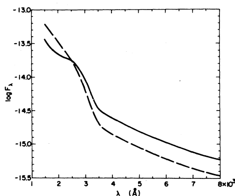
Figure 4. Smoothed energy distribution of the H-H 2H continuum in the range 1300 Å to 8000 Å, dereddened using the Seaton (1979) (dashes) and the Bohlin and Savage (1981) \Theta Ori extinction curve (solid line). This is a slightly modified form of figure 3, published by Böhm-Vitense et al. in Ap.J. 262, 224 (1982).
