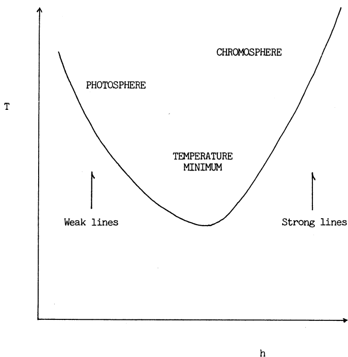
Figure 1. Schematic temperature profile showing temperature rise above the photosphere corresponding to the chromosphere. Arrows show regions where weak and strong lines form.
