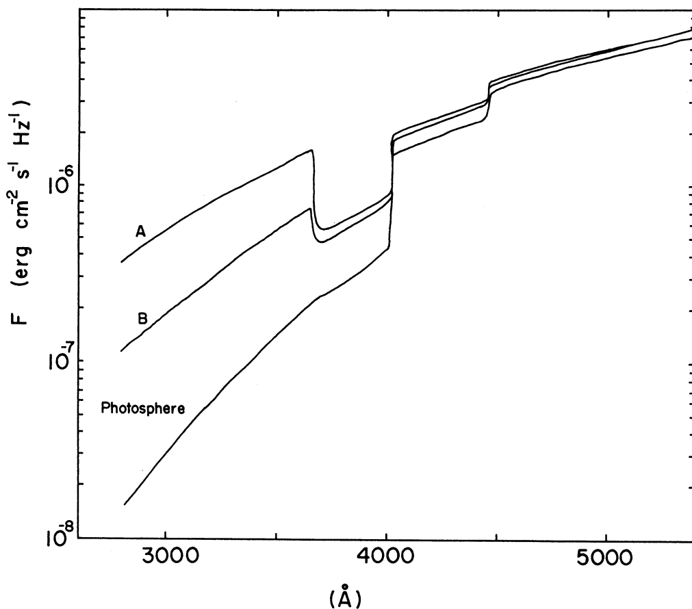
Figure 3. Continuum energy distribution for models A and B of Figure 2. The photospheric flux is also shown for comparison.
