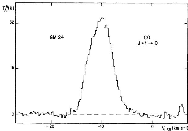
Fig. 6. Spectrum of the J = 1 → 0 CO transition for the central position of the cometary nebula GM 24. The velocity resolution is 0.26 km s -1 .
