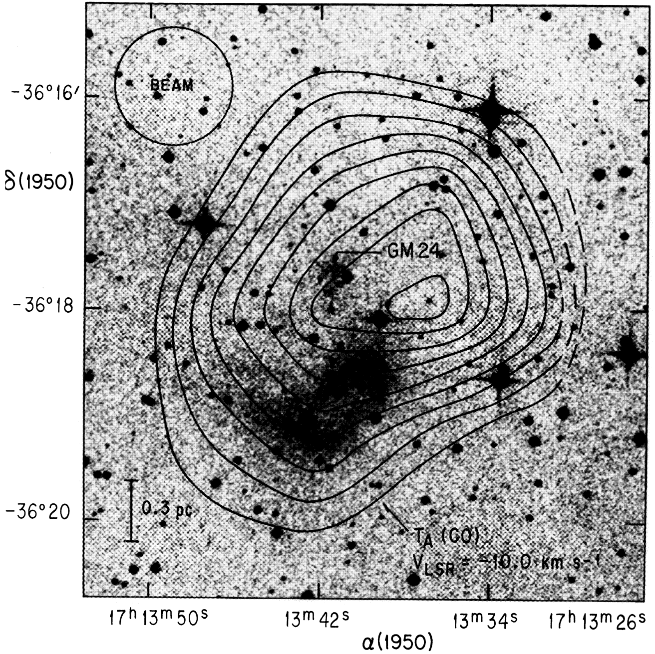
Fig. 7. Contour map of the antenna temperature of the J=1 \rightarrow 0 CO transition at V_{\text{LSR}} = -10.0 \text{ km s}^{-1} superposed on an optical photograph of the GM 24 region. The lowest contour is 25 K and the increment is 1 K.
