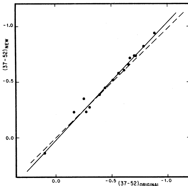
Fig. 1. The average values of (37-52) observed with the new 13C filters (set No. 1) are plotted against the original (37-52) values of Schuster and Alvarez (1983) for 16 Be stars. The photometrically most variable Be stars of Alvarez and Schuster (1982) have been excluded. The dashed line has a slope of unity, and the solid line is a least-squares fit to the data.
