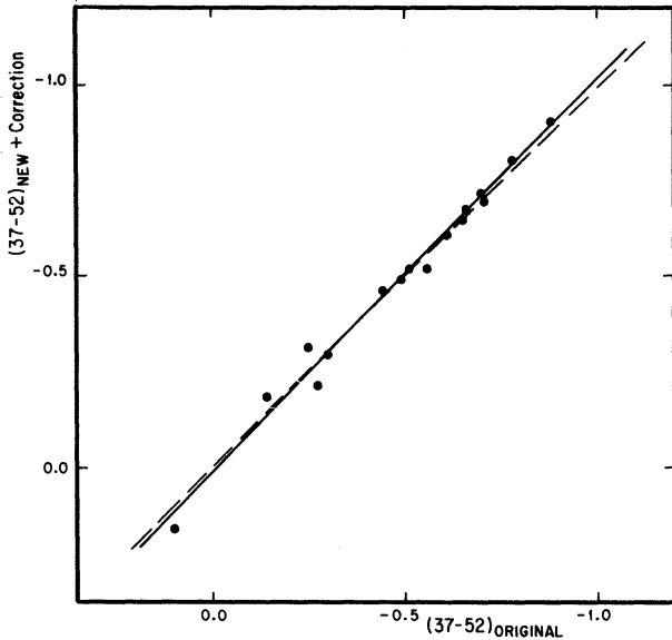
Fig. 2. The same as Figure 1 except that the new (37-52) values have been corrected using the first solution given in the text. This is the solution number 5 of Schuster and Guichard (1984) which corrects for the transformation residuals of normal B-type stars, luminosity classes V-III.
