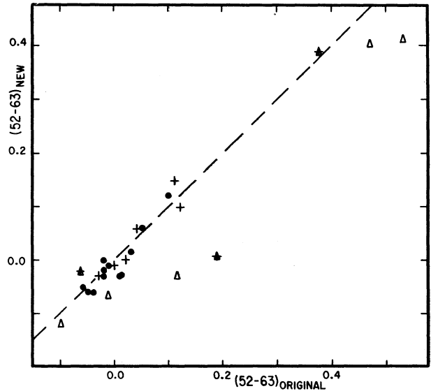
Fig. 3. The (52-63) values observed with the new 13C filters are plotted against the original (52-63) values of Schuster and Alvarez (1983). Be stars with strong emission lines (Hubert-Delplace 1976) are shown as triangles, the photometrically more variable Be stars (Alvarez and Schuster 1982) by pluses, and other Be or shell stars by circles.
