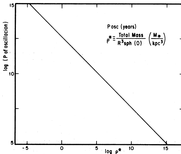
Fig. 3. The relationship between the period of oscillation, P , and the average density.
