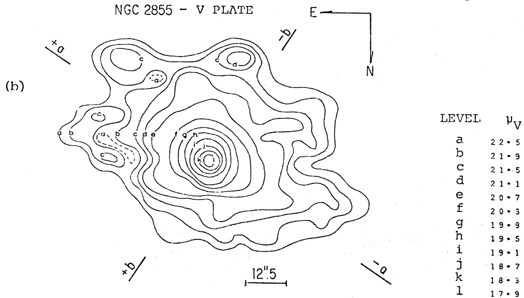
Fig. 1. Isophotes of NGC 2855 from OAB plates 213 (B) (a) and 214 (V) (b). Magnitudes levels are identified. Directions a and b are along the major and minor axes of the galaxy.
