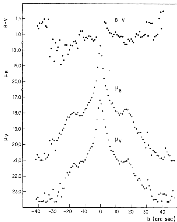
Fig. 5. Plots of (B-V) , B and V luminosity profiles versus radius along major axis of NGC 4507.
