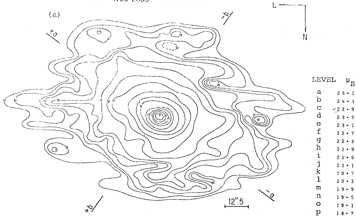
NGC 2855 - V PLATE
