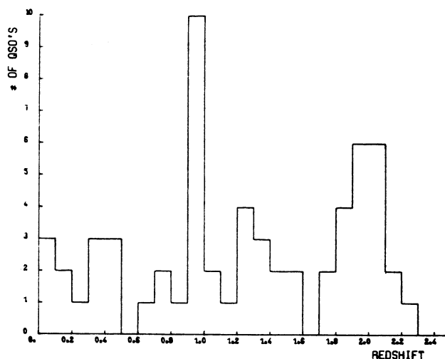
Fig. 1. Redshift distribution for 61 quasars.
