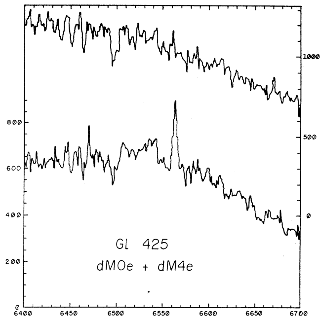
Fig. 2. H \alpha Intensified Reticon Spectra of both components of the pair Gl 425 at 90 Å/mm, in counts/pixel vs. wavelength. Continuum curvature is due to the detector response. The upper spectrum is from the brighter component.
