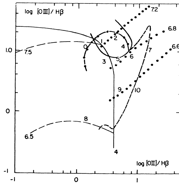
Figure 1 - [OIII]\lambda\lambda(5007+4959)/H\beta versus [OII]\lambda 3727/H\beta . Thin lines correspond to photoionization models: solid line is labelled by \log n_H and dashed lines by \log U . Thick lines correspond to composite model (photoionization and shock): solid line gives the ejection model results and dotted - dashed line refers to infalling model; dashed line correspond to shock dominated case. Dotted lines give the results of coupled photoionization and relativistic electrons effects, and are labelled by the corresponding \log U values. The position of each group of galaxies is also indicated.
