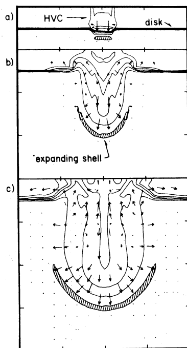
Fig. 3. Numerical simulation for the collision of a HVC and the plane. Arrows indicate the velocity field (units are arbitrary; adapted from Tenorio-Tagle et al. 1985)
