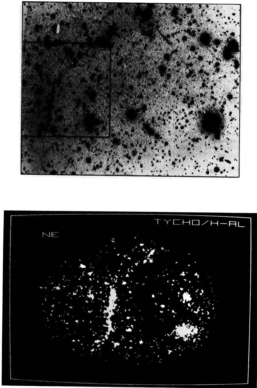
Fig. 3. Optical image of Tycho's SNR. The upper picture is from van den Bergh et al. (1973), and the area within the square is the same region covered by the MEPSICRON image shown in the lower part of this figure.
