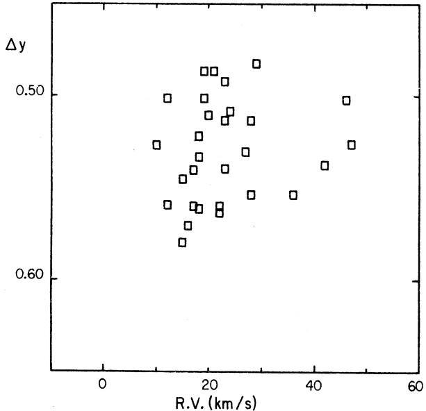
Fig. 4. The y magnitude differences plotted as a function of the C IV radial velocities.
