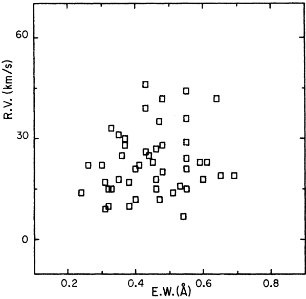
Fig. 5. The C IV radial velocities plotted as a function of the C IV equivalent widths.
