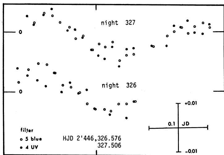
Fig. 3. Photometry of LQ And obtained on September 1985 with narrow filters UV: ( \lambda 3490 Å) and B: ( \lambda 4740 Å). No color variation is clearly observed. Observed amplitude for this star is \approx 20 - 30 m mag. This figure and also Figure 4 have been adopted from Sareyan et al. (1986).
