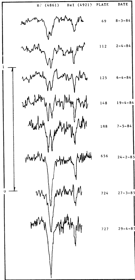
Fig. 1a: H \beta and HeI 4921 line profiles of \mu Cen in March 1984 to April 1985.
