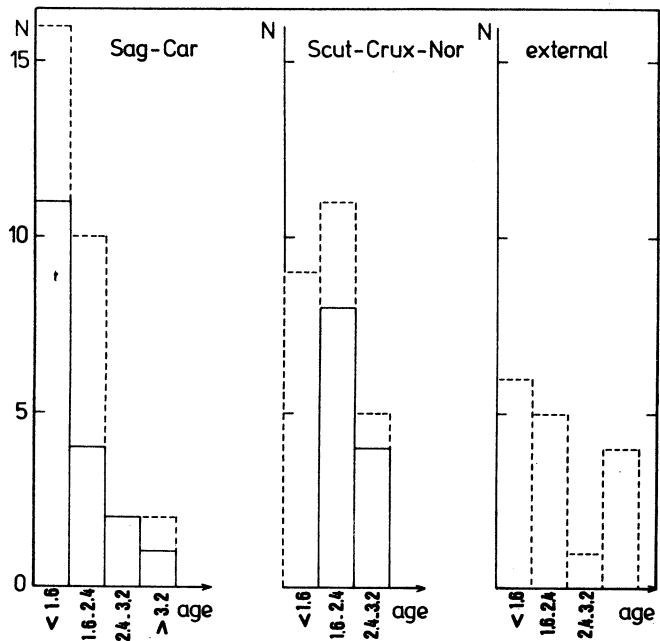
Fig. 6. The distribution of ages for the three arms. The dashed line represents regions with U \geq U_{\text{orion}} (= 72 \text{ pc cm}^2) . The Centaurus spur is included in the Sag-Car arm (see text). The full line represents only regions with U \geq 110 \text{ pc cm}^2 .
