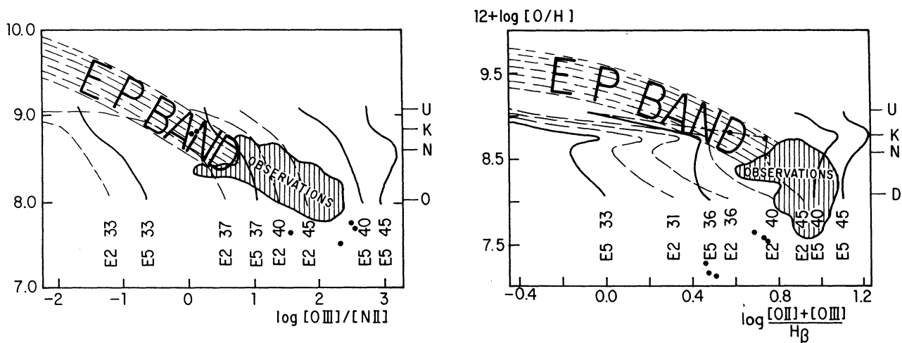
Figs. 9a,b: Iso-temperature-density curves, from Rubin's (1985), were superposed to a sketch of the EP relation for [O III]/N II and [O II] + [O III]/H\beta in order to show the direction of the evolution. 90% of the observations quoted by EP are within the dashed areas, and the rest is shown as points. EP bend is 0.2 dex bend around EP mean relation.
