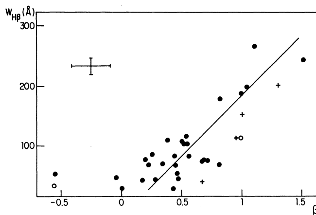
Fig. 7. WH_\beta vs. (2 \log DHII/Dass) , where DHII and Dass are the diameters of ionized region and ionizing association \bullet = LMC, \circ = SMC, and + = M33.
