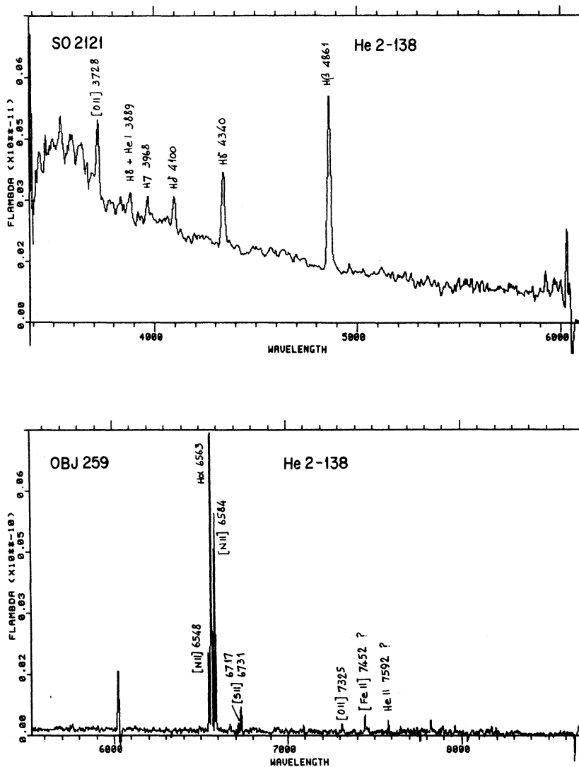
Fig. 2. The same as Figure 1 for the low excitation PN He2-138. The spectra correspond to the whole nebula.
