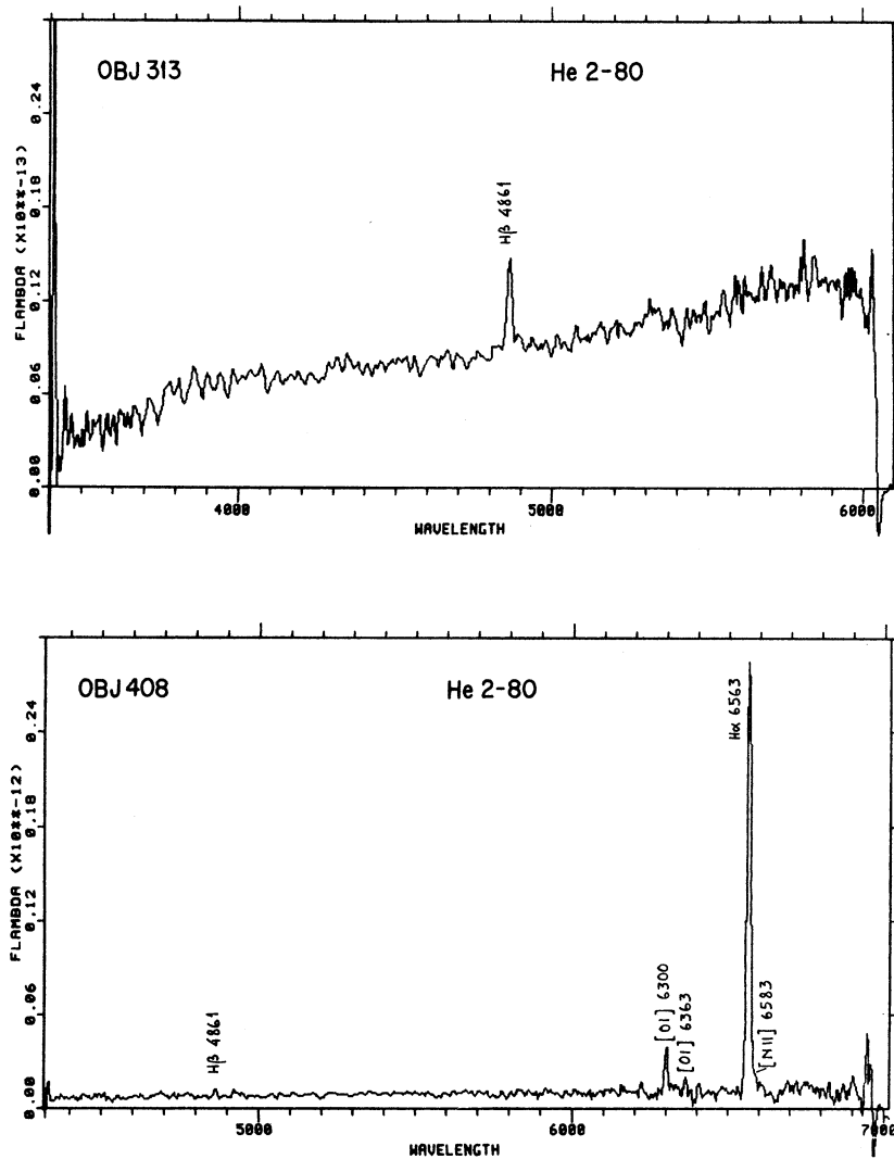
Fig. 3. The same as Figure 2 for the object He2-80, probably not a PN according to Webster (1966). The spectral ranges covered in this case are \lambda\lambda 3400-6000 Å and \lambda\lambda 4300-7000 Å.
