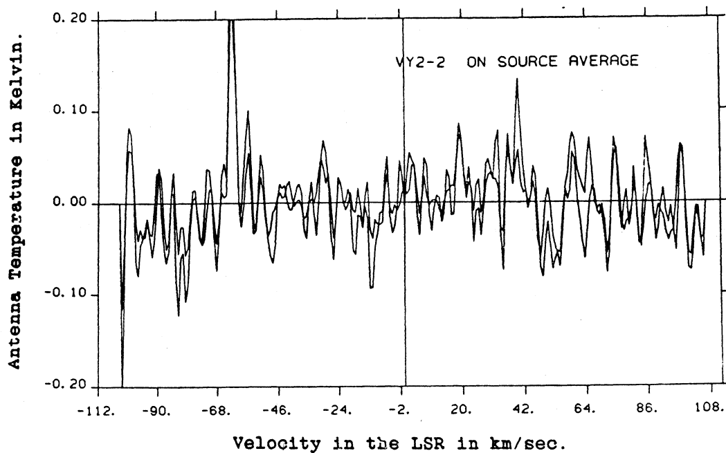
Fig. 3. VY 2-2, 1667.253 MHz. Both polarizations shown. 22 minutes total integration time, rms is .039 K.
