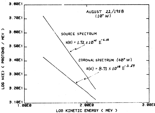
Fig. 5. Coronal Spectrum.
