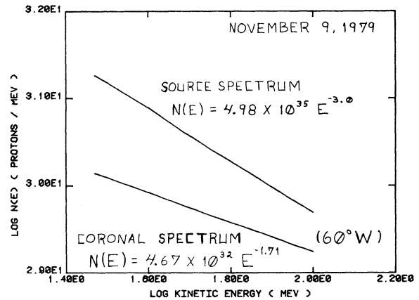
Fig. 8. Coronal Spectrum.
