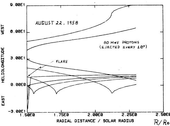
Fig. 4. Trajectories of Protons.
