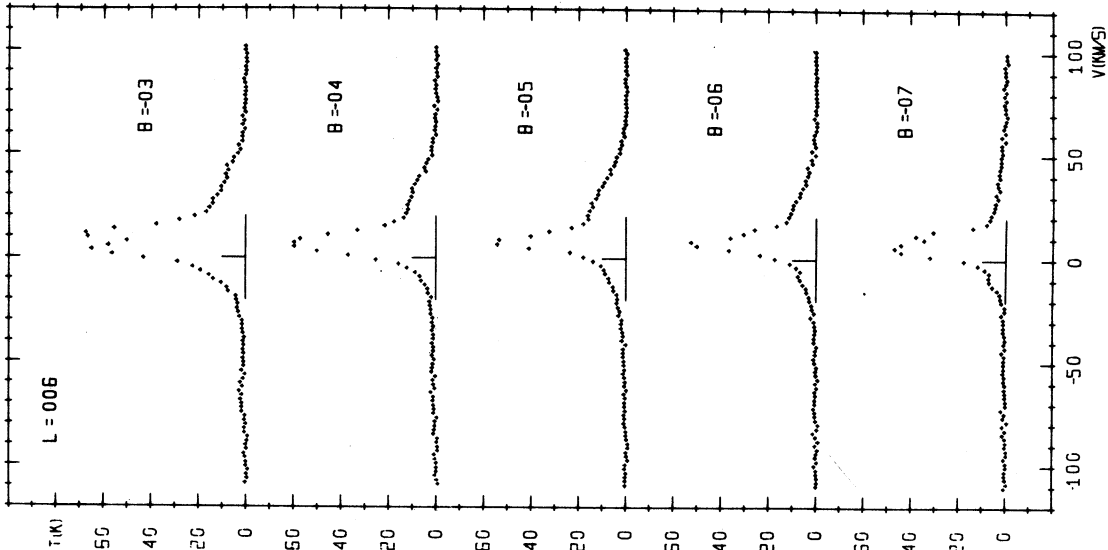
Fig. 19. Observed profiles for l = 6^\circ
