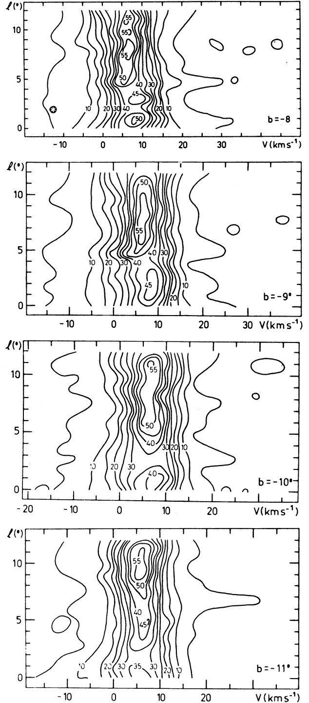
Figs. 45 to 48 Contour maps in the plane l - v for b = -8^\circ , -9^\circ , -10^\circ , and -11^\circ .
