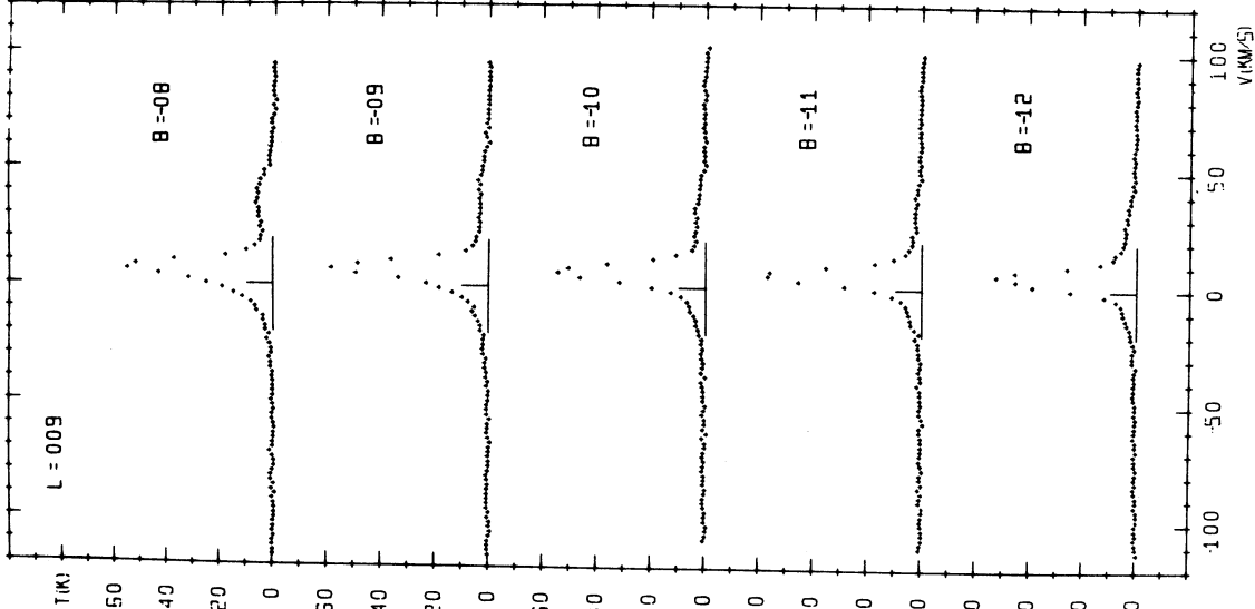
Fig. 11. Observed profiles for l = 9^\circ
