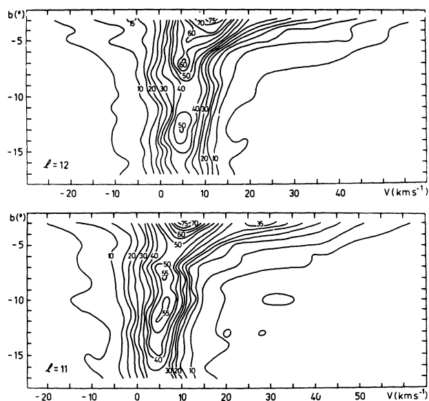
Figs. 55 to 56. Contour maps in the plane b - v for l = 12^\circ and 11^\circ .
