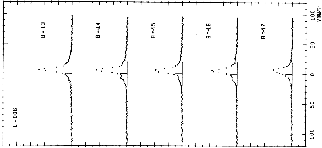
Fig. 21. Observed profiles for l = 6^\circ
