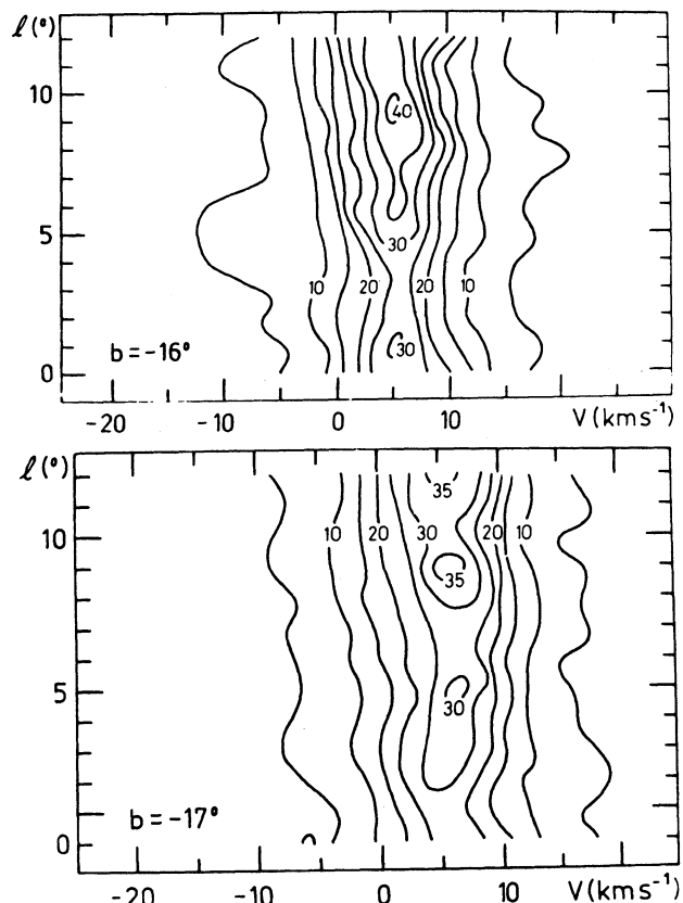
Figs. 53 to 54. Contour maps in the plane l - v for b = -16^\circ and -17^\circ .
