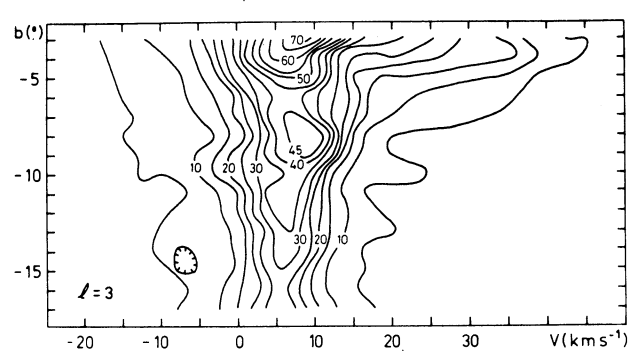
Figs. 61 to 64. Countour maps in the plane b - v for \ell = 6^\circ , 5^\circ , 4^\circ , and 3^\circ .
