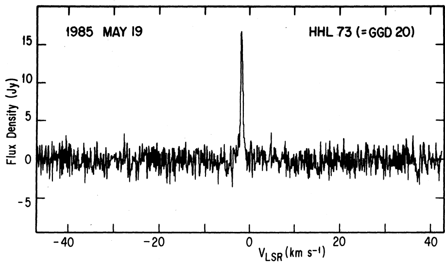
Fig. 3. Spectrum of the water maser associated with HHL73 (GGD20). The velocity resolution is 0.22 km s -1 .
