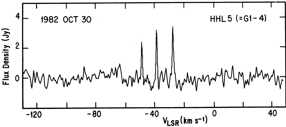
Fig. 1. Spectrum of the water maser associated with HHL5 (= G1-4). The velocity resolution is 1.8 km s -1 . This source is associated with CRL437.
