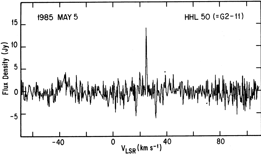
Fig. 2. Spectrum of the water maser associated with HHL50 (G2-11). The velocity resolution is 0.88 km s -1 . This spectrum was obtained with the frequency-switching technique. This technique produces the two apparent “absorption” features symmetrically displaced with respect to the emission line.
