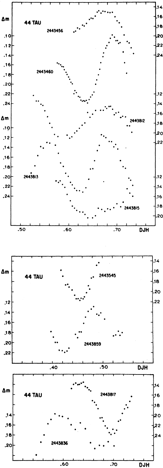
Fig. 1. Light curves of 44 Tau in 1977 and 1978, in filter B.
