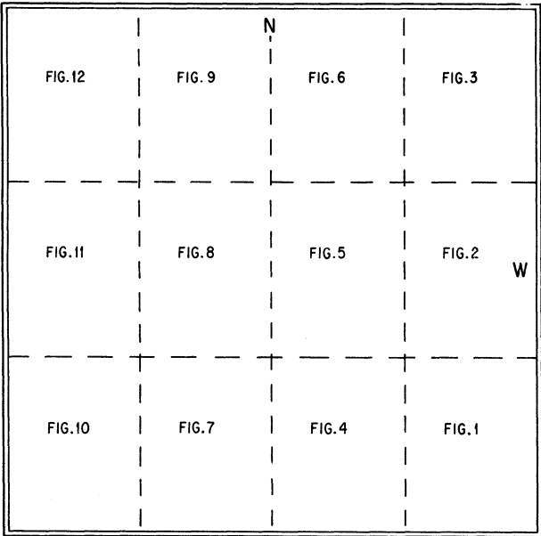
Fig. I. A rough diagram showing the distribution of the figures or charts which cover the whole field of the Mount Palomar 48-inch Schmidt telescope, centered at 0^h53^m and -11^\circ.5 (1950). It is convenient to emphasize that there exists a big overlap between the 12 different figures. In all cases North is at the top and West to the right.
