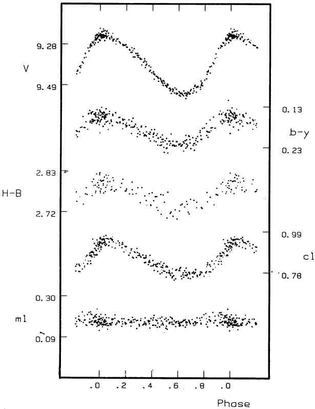
Fig. 2. Light-curves of AD CMi.
