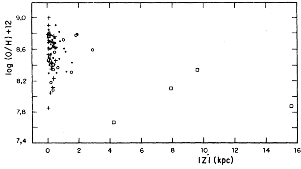
Fig. 3. The same as Figure 2 for oxygen.
