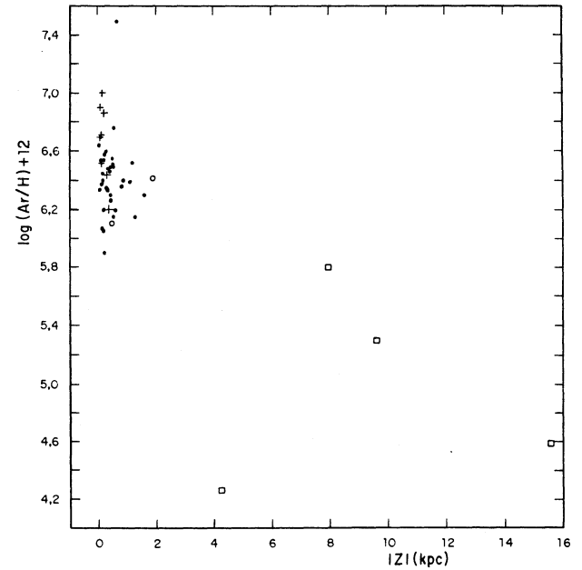
Fig. 8. The same as Figure 2 for argon.
