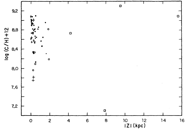
Fig. 6. The same as Figure 2 for carbon.
