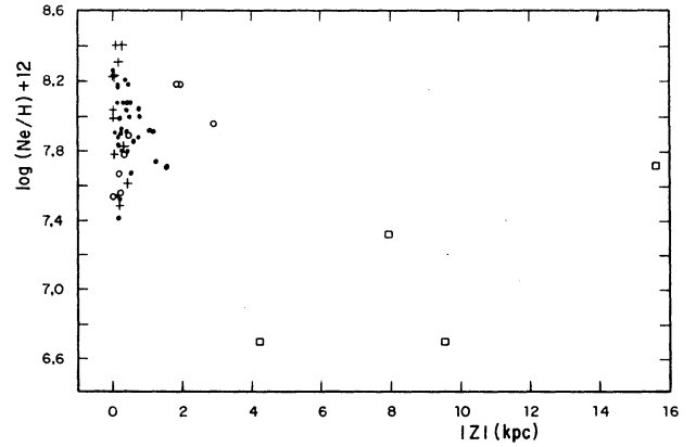
Fig. 7. The same as Figure 2 for neon.
