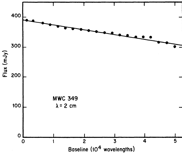
Fig. 1. Visibility data (flux versus baseline) for the 2-cm continuum from MWC349. The solid line is the linear fit described in the text.
