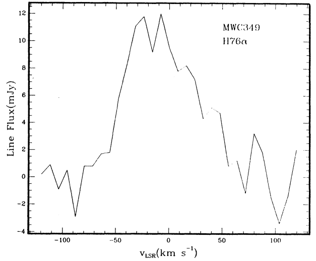
Fig. 2. Spectrum of the H76 \alpha line emission from MWC349. The velocity resolution is 8 \text{ km s}^{-1} .
