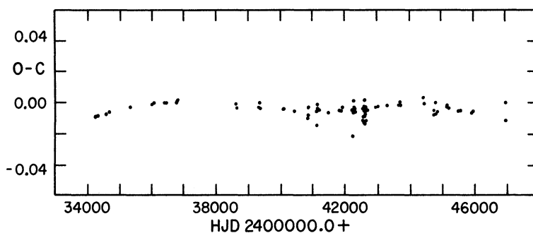
Fig. 5. O-C versus HJD, using the quadratic ephemeris \text{HJD } 2436744.4195 + 0.409640403 E + (3.40923) E^2/2 with the period and rate of change of the period deduced in the present paper.
