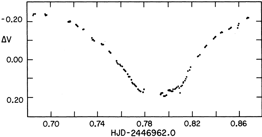
Fig. 1. Light curve of V566 Ophiuchi corresponding to the night of June 15 – 16, 1987. ΔV is given in magnitudes.
