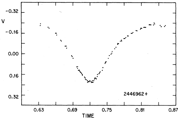
Fig. 2. Light curve of the W Uma star V502 Ophiuchi for the night HJD 2446962. The horizontal axis zero is arbitrary due to a problem in the clock setting at the beginning of the night. This light curve is shown merely to study the amplitude variation behaviour.
