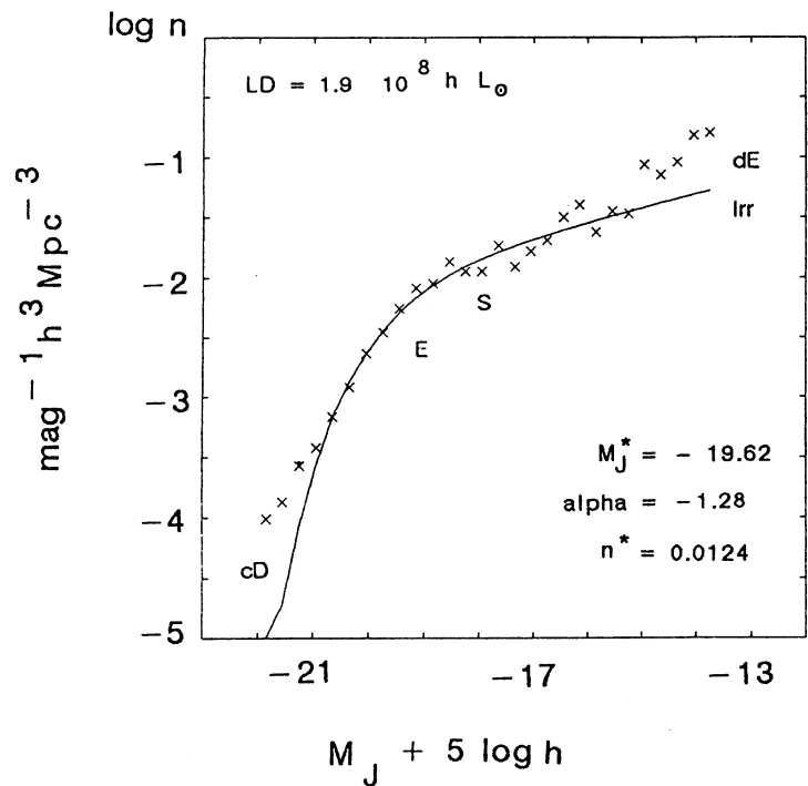
Fig. 2. The general luminosity function obtained from 40 000 galaxies in the vicinity of the South Galactic Pole up to z = 0.3 . Deviations from the Schechter fit seem to be real. The letters indicate galaxy types, the lower inserts are the parameters of the Schechter fit (line), the upper insert gives the mean luminous density (Schuecker 1989).
