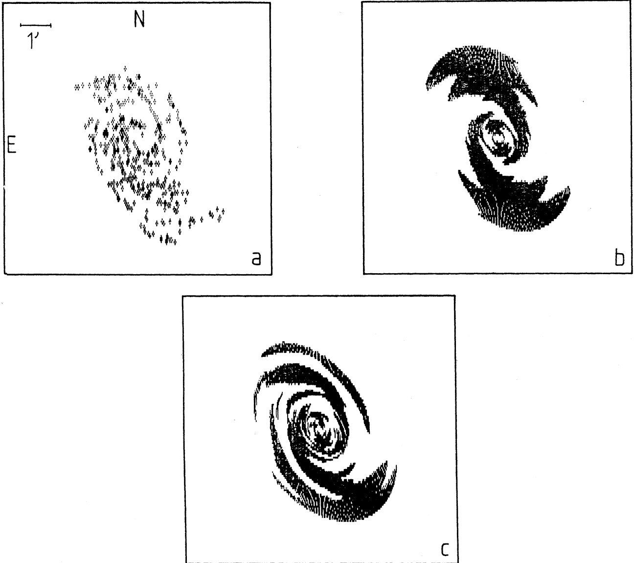
Fig. 4 a. The galaxy. b) m = 2 component. c) Sum of main components ( m = 1, 2 , and 4).
