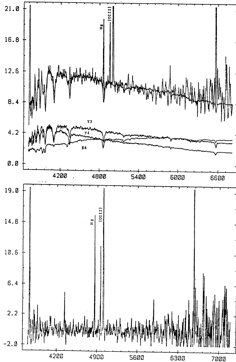
Figure 3.- The 24''S region is similar to the 24''N one. The flux fraction from the old component is considerably larger than in the nuclear region. Notice that after subtraction, Balmer emission lines are enhanced.
