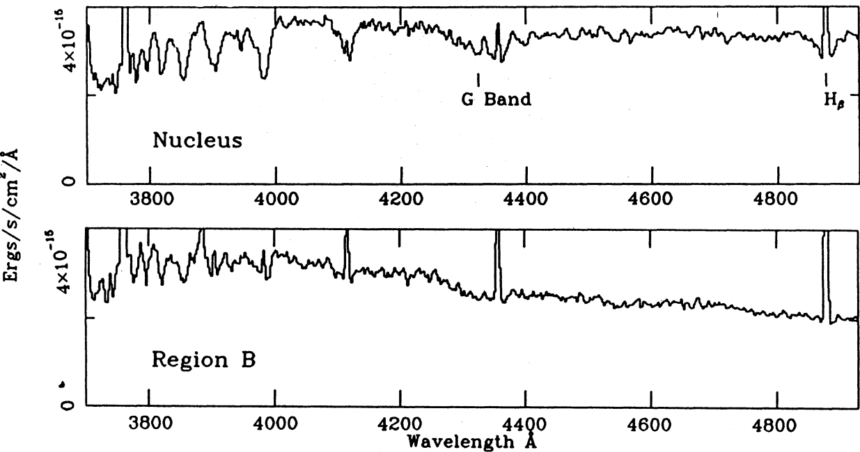
Fig. 3. Blue ( \lambda 3700 - 5000 \text{ \AA} ) spectra for a) the nucleus and b) region B. Strong emission lines are out of scale.
