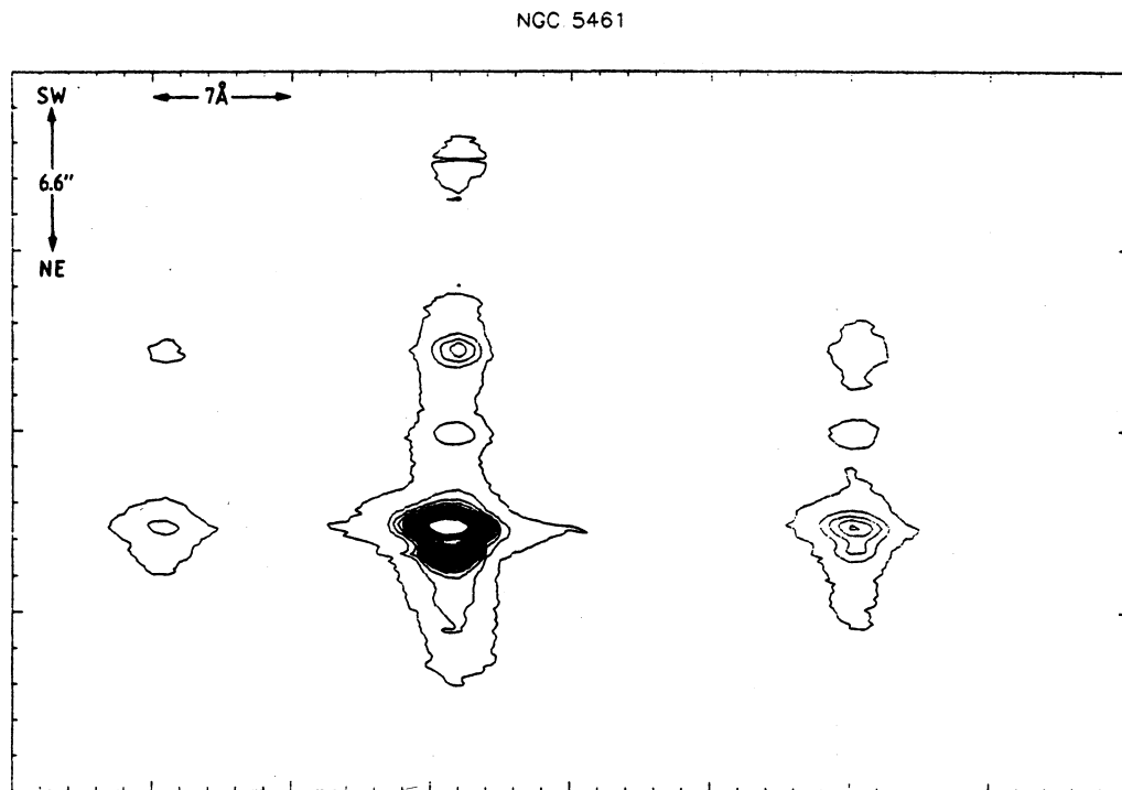
Figure 1: Contour plots of H\alpha + [\text{N II}] \lambda\lambda 6548, 6584 for the long slit spectrogram of NGC 5461. The slit is oriented along the major axis of the region. Position Angle is 66^\circ .
