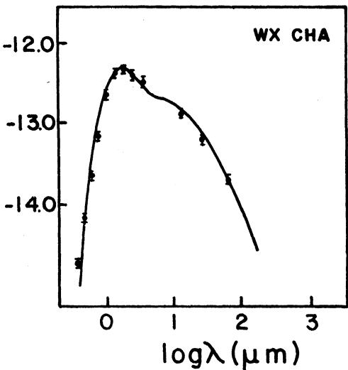
Figure 2: Energy distribution of WX Cha
