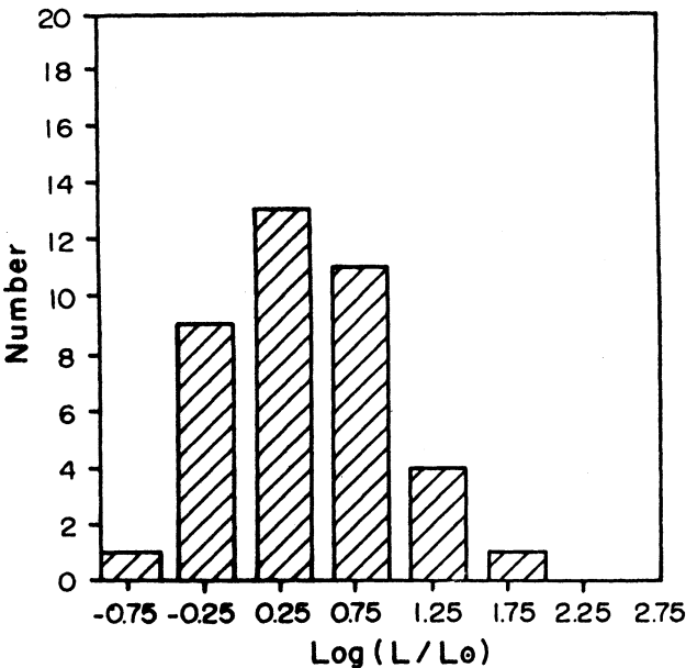
Figure 3: Luminosity function of Cham I members
