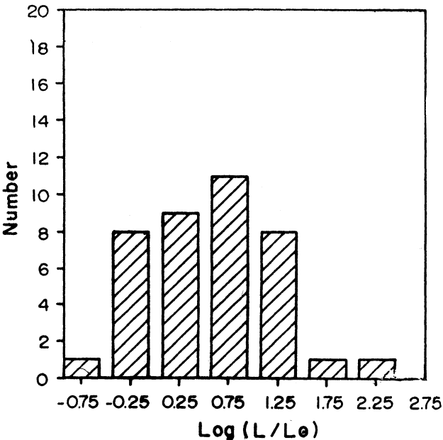
Figure 4: Luminosity function of Rho Ophiuchi members
