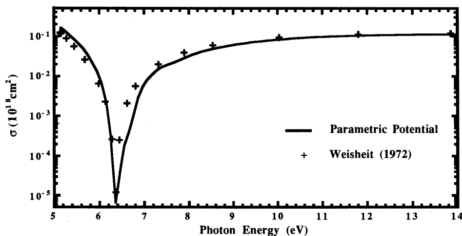
Figure 2 --- Photoionization cross section of 3s electron in neutral sodium
