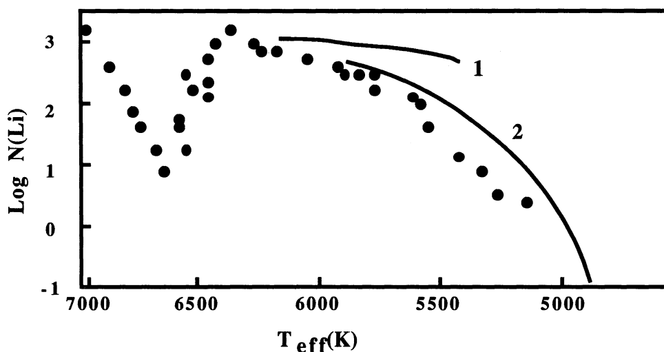
Figure 8 --- Lithium abundances are plotted versus star surface temperatures where the initial value is \text{Log } N(\text{Li}) = 3.2 and the scale \text{Log } N(\text{hydrogen}) = 12 is used. Curve 1: Cox and Tabor (1976) ; Curve 2: OPAL ; •: observations.
