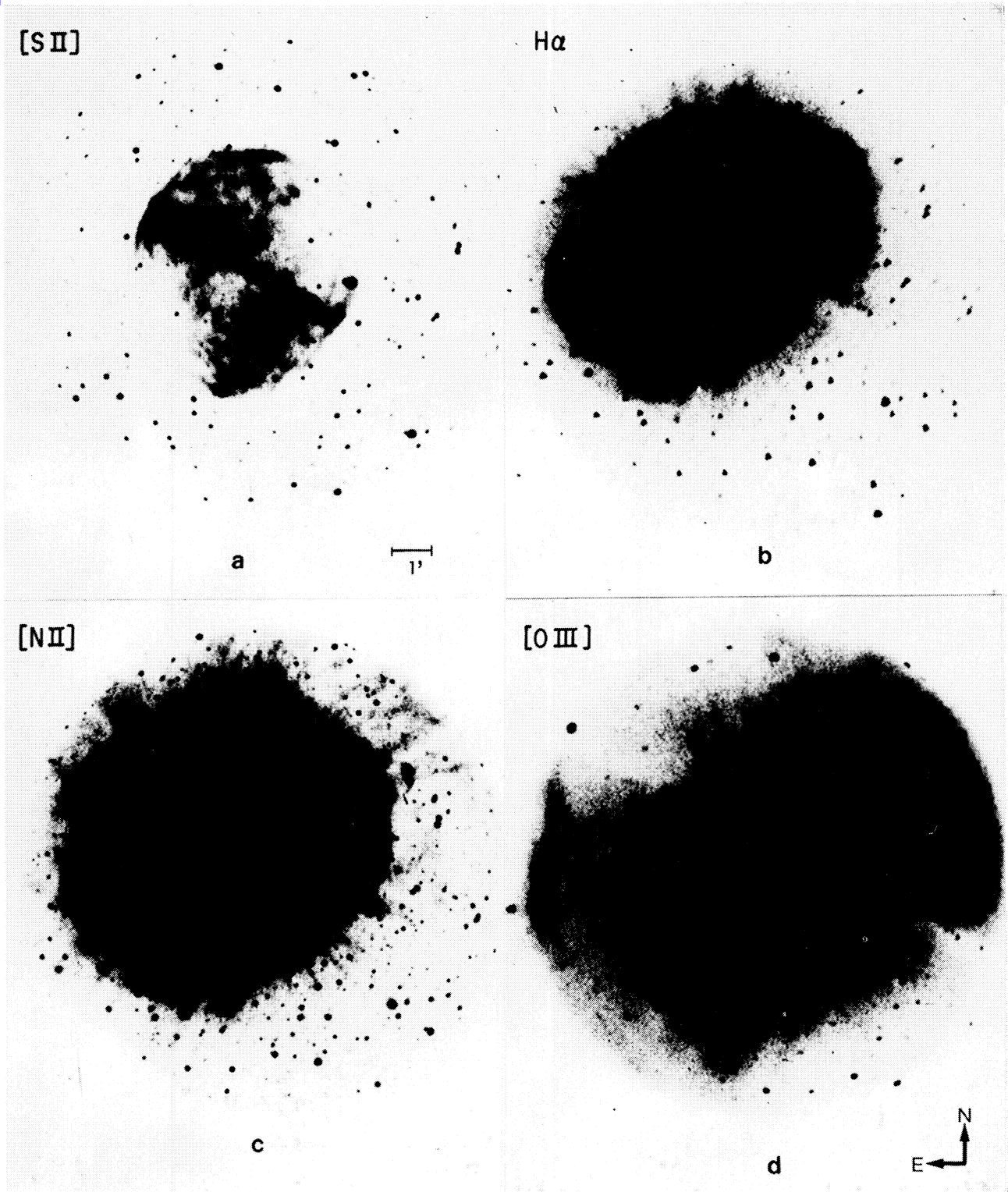
Fig. 1. Monochromatic images of M27. The scale and orientation are the same from a to d.
