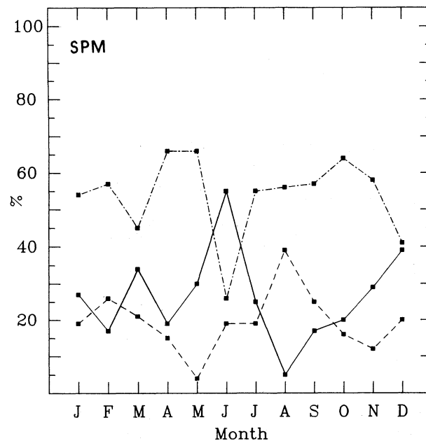
Fig. 4. Monthly fraction of nights of low (continuous line), intermediate (broken line) and high (dotted line) relative humidity, according to the definitions given in §II.
