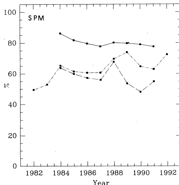
Fig. 6. Yearly fraction of nights of photometric (broken line) and of spectroscopic quality (continuous line) in San Pedro Mártir during the period January 1984 to December 1991. The dotted line marks the actual use of the 2.1-m telescope (excluding the time lost due to telescope/instrument failure) in the period July 1982 to June 1992.
