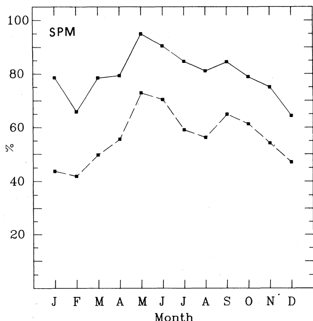
Fig. 5. Monthly fraction of nights of photometric (broken line) and of spectroscopic quality (continuous line) in San Pedro Mártir during the period January 1984 to December 1991.
