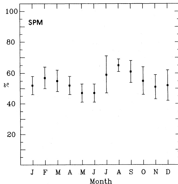
Fig. 3. Monthly mean relative humidity near the ground and its standard deviation in San Pedro Mártir.
