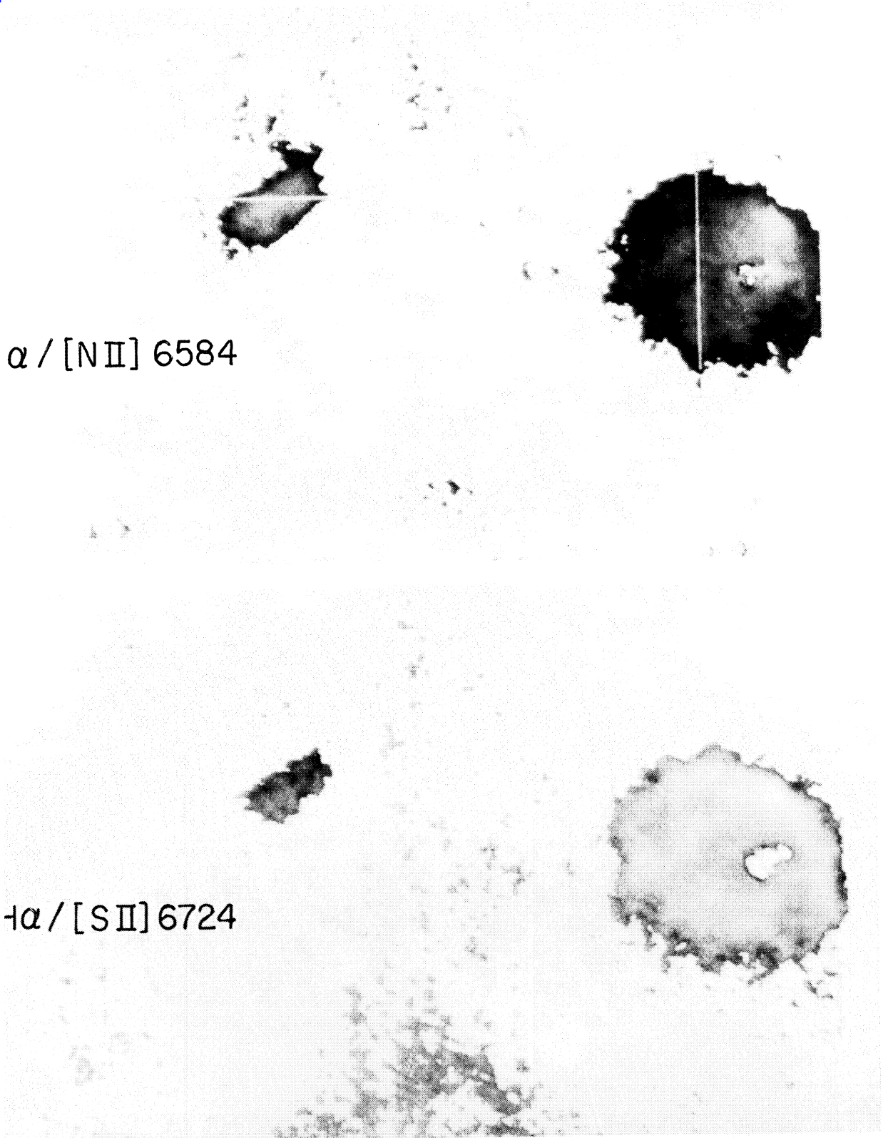
Fig. 2. (a) \text{H}\alpha/[\text{N II}] line ratio image. (b) \text{H}\alpha/[\text{S II}] line ratio image.
