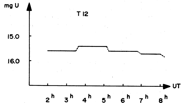
Fig 3. Light curve of slow flare of star T12.
