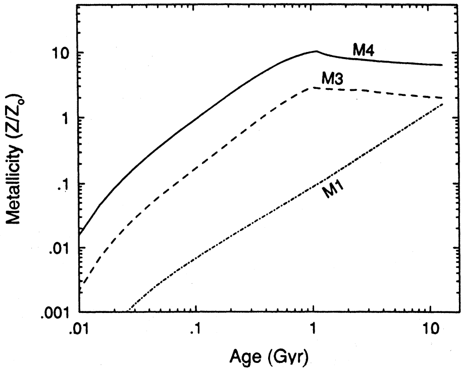
Figure 6. Metallicity vs. Age in 3 chemical evolution models.
