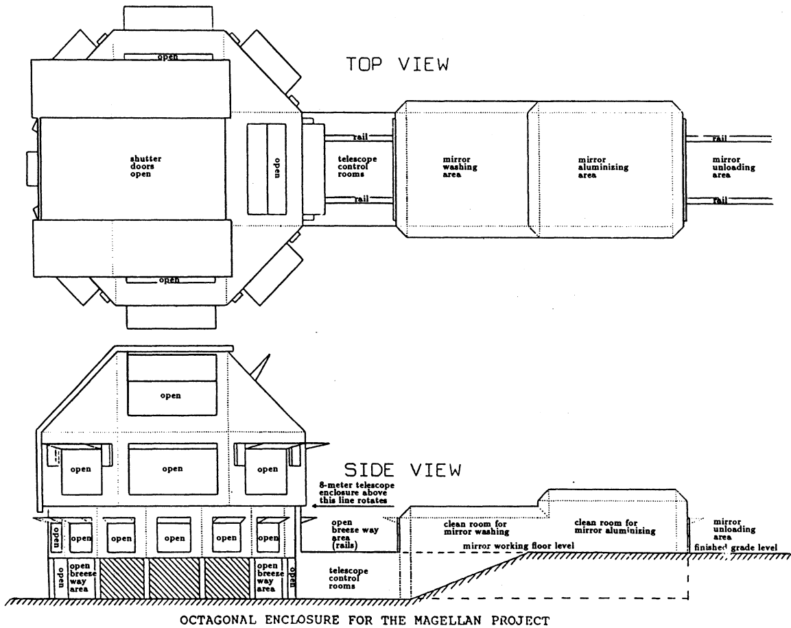
Fig. 2. Conceptual design of the enclosure for the telescope. Notice all the ports marked "OPEN". The auxiliary building to the right of the dome can be used for the same purposes for a second telescope placed to the right of the picture.
