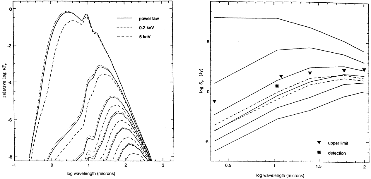
Fig. 1. — (a) The relative energy spectra arising from dust irradiated by 3 different x-ray continua at flux levels of 10^8, 10^4, 10^2, 10, 1, 0.1 erg \text{cm}^{-2} \text{s}^{-1} (top to bottom). (b) The predicted near- to far-infrared spectra for the \lambda 10.8\mu\text{m} features. The solid lines are computed from the power-law models, with the highest flux level at the top, as in (a). The filled triangles indicate upper limits for the K band and four IRAS bands. The filled square is the detection of Telesco & Decher (1988). The dashed lines correspond to flux levels of 10^{1.1} and 10^{0.6} erg \text{cm}^{-2} \text{s}^{-1} and include an additional UV component as explained in the text.
